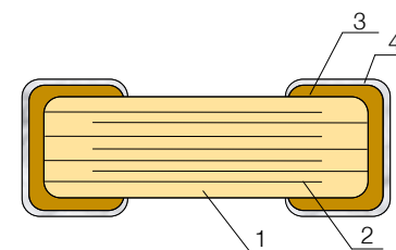
AgPdCu Termination
