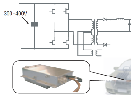
DC-DC Converters for Hybrid Electric Vehicles
