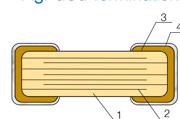
AgPdCu Termination
