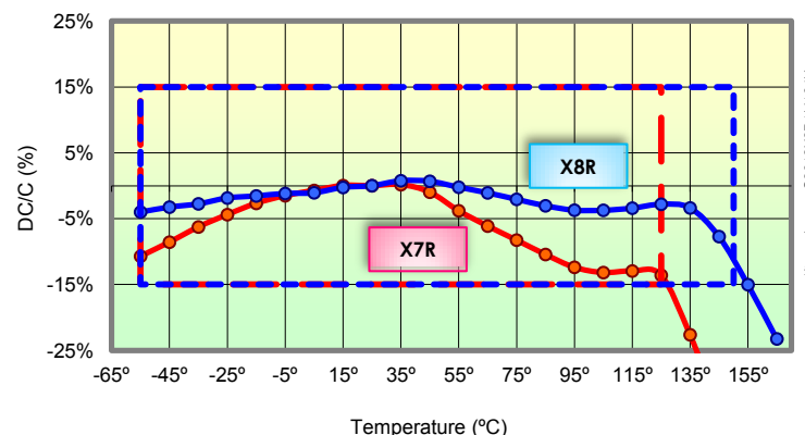
Temperature Characteristic Curve (X7R vs. X8R)
