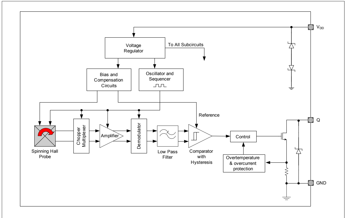
Figure 2-2 Functional Block Diagram TLE4964-4M
