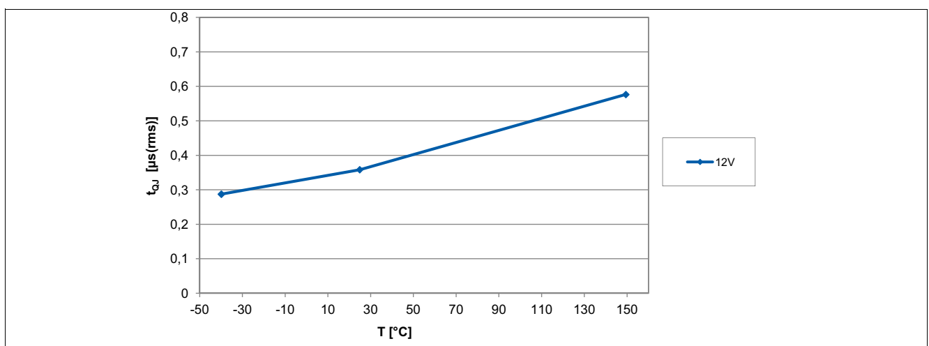
Figure 6-15 Output Signal Jitter of the TLE4964-4M over Temperature
