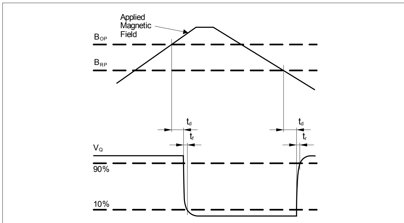
Figure 2-3 Timing Diagram TLE4964-4M
