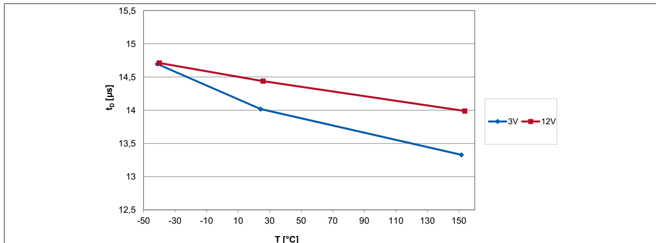
Figure 6-2 Signal Delay Time of the TLE4964-4M over Temperature
