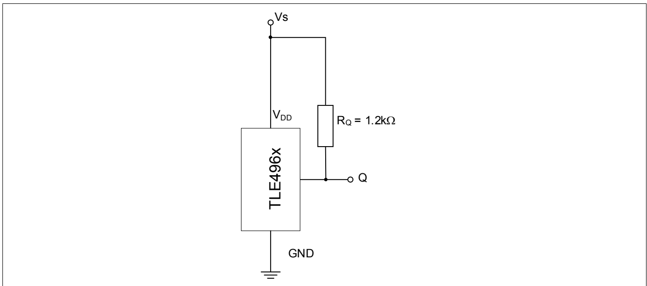
Figure 3-1 Basic Application Circuit #1: Only Pull-Up Resistor is necessary
