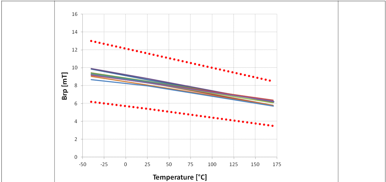
Figure 5-2 Release Point ( B_{RP} ) of the TLE4964-4M over Temperature
