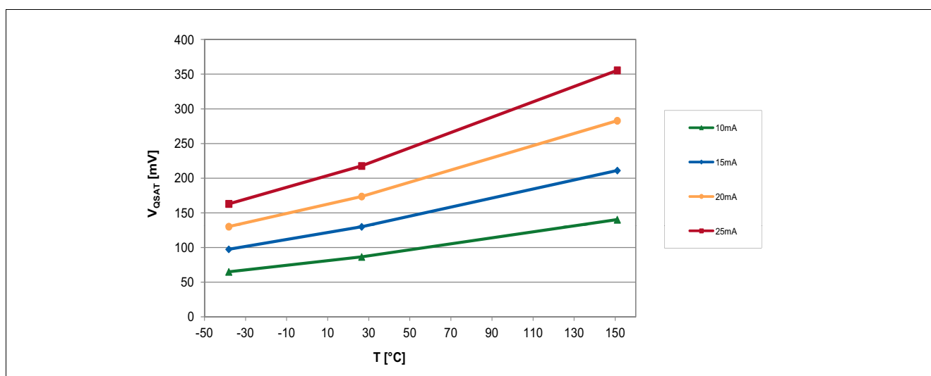
Figure 6-12 Saturation Voltage of the TLE4964-4M over Temperature
