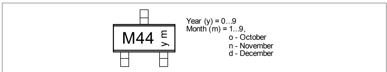
Figure 4-5 Marking of TLE4964-4M
