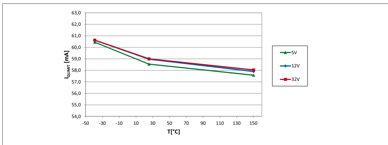
Figure 6-5 Output Current Limit of the TLE4964-4M over Temperature
