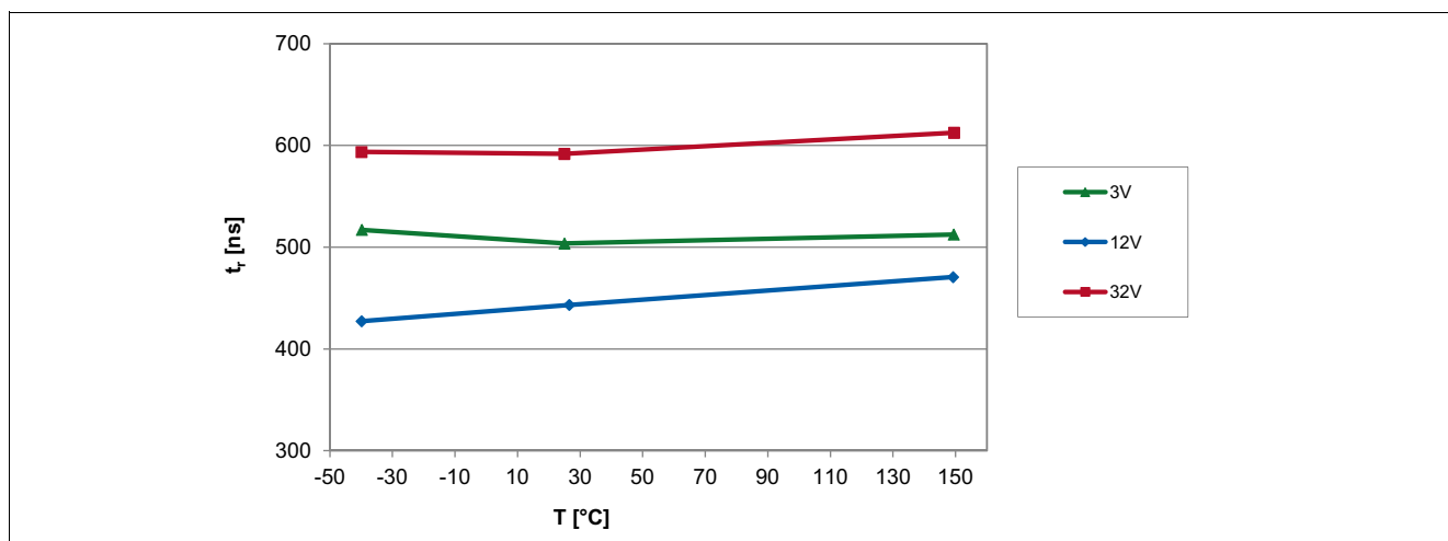
Figure 6-9 Output Rise Time of the TLE4964-4M over Temperature
