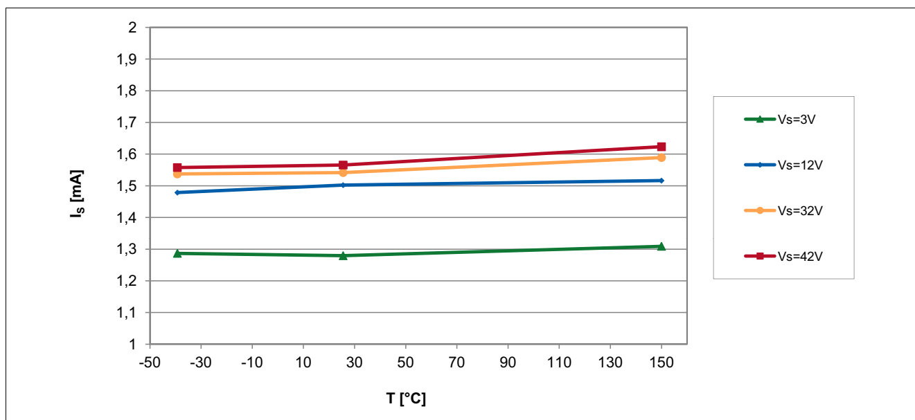
Figure 6-3 Supply Current of the TLE4964-4M over Temperature
