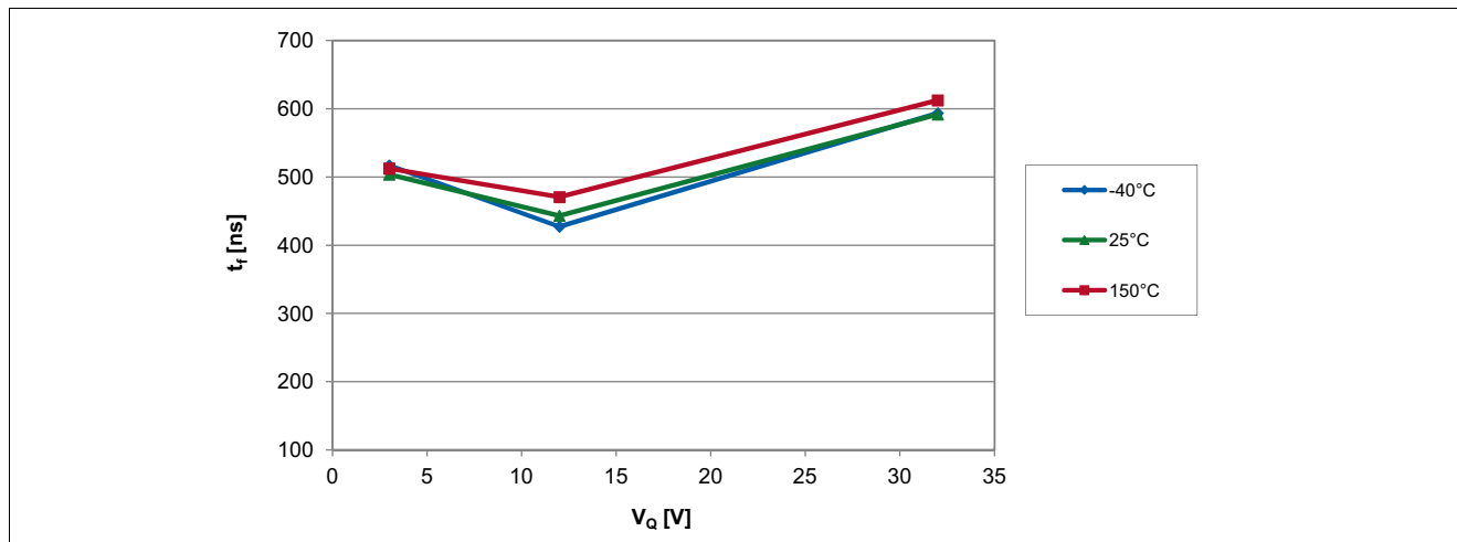
Figure 6-10 Output Rise Time of the TLE4964-4M over applied Pull-up Voltage
