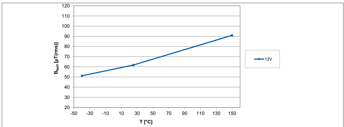
Figure 6-14 Effective Noise of the TLE4964-4M Thresholds over Temperature
