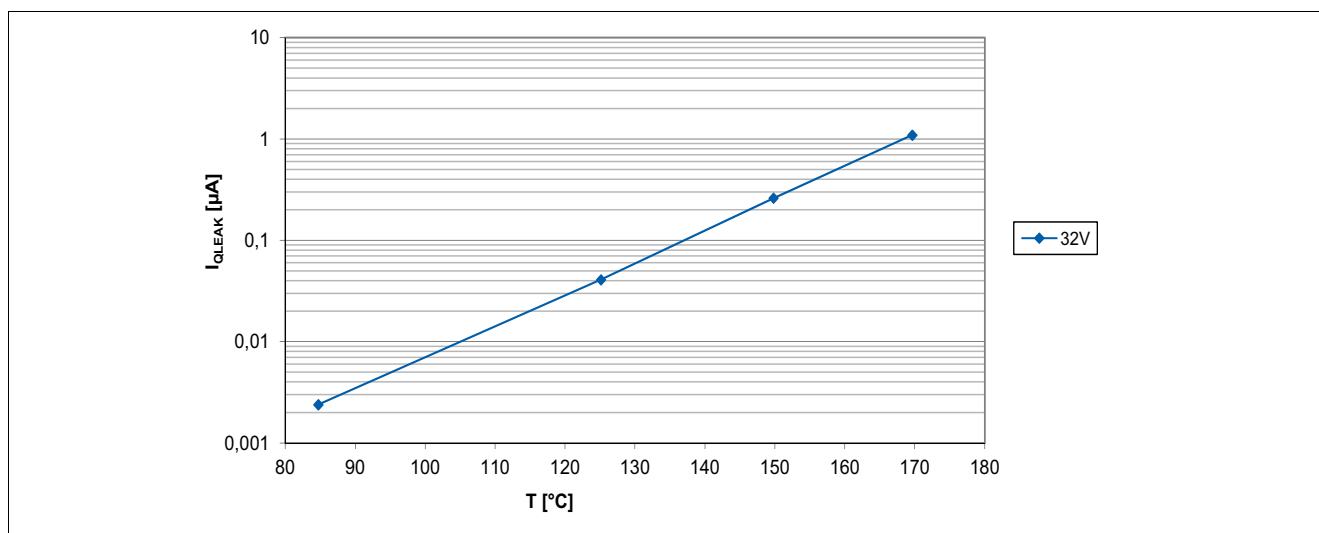
Figure 6-11 Output Leakage Current of the TLE4964-4M over Temperature
