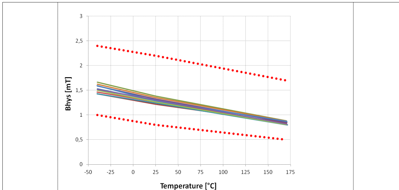
Figure 5-3 Hysteresis ( B_{Hys} ) of the TLE4964-4M over Temperature
