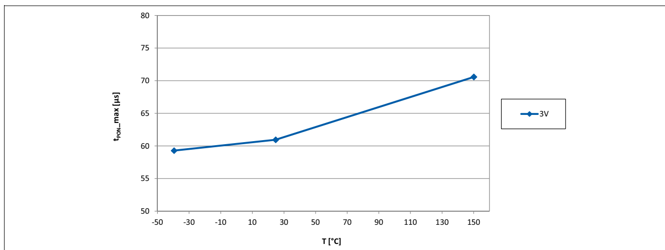
Figure 6-1 Power On Time t_{PON} of the TLE4964-4M over Temperature
