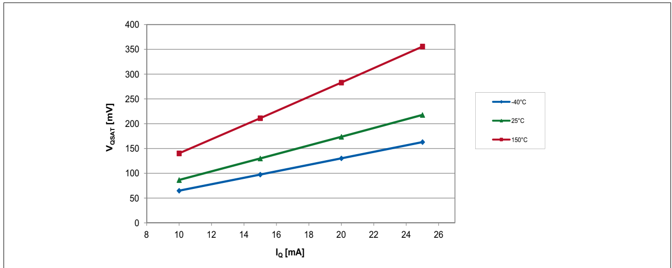
Figure 6-13 Saturation Voltage of the TLE4964-4M over Output Current
