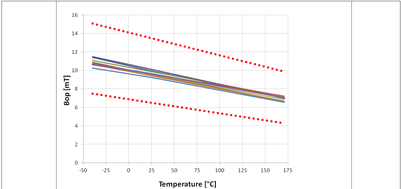
Figure 5-1 Operating Point ( B_{OP} ) of the TLE4964-4M over Temperature
