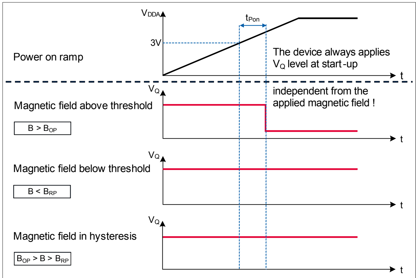
Figure 2-5 Illustration of the Start-up Behavior of the TLE4964-4M
