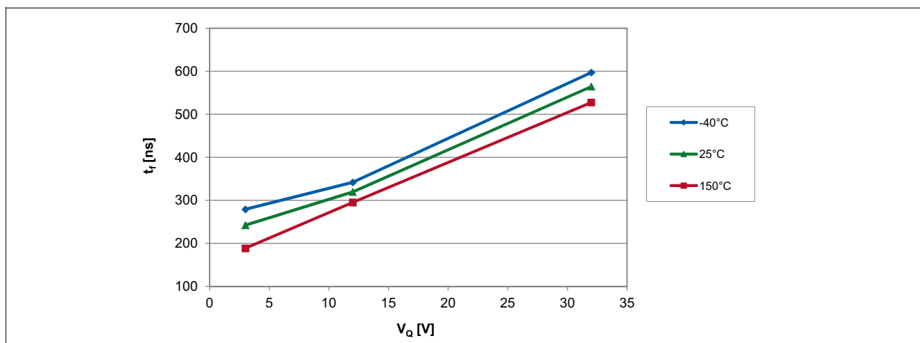
Figure 6-8 Output Fall Time of the TLE4964-4M over applied Pull-up Voltage
