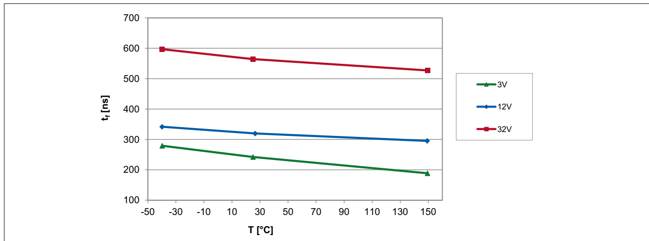
Figure 6-7 Output Fall Time of the TLE4964-4M over Temperature
