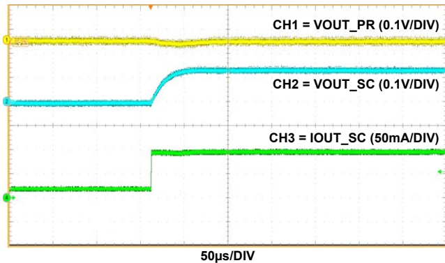
Figure 18. Loading Transient ( V_{IN} = 24V , V_{OUT\_PR} = 5V , V_{OUT\_SC} = -5V at I_{OUT\_PR} = 0A , I_{OUT\_SC} = 25mA to 75mA, 700kHz, FCCM)
