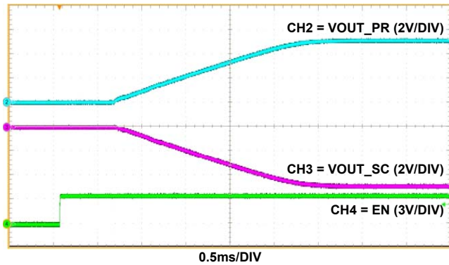
Figure 16. Start-Up by EN ( V_{IN} = 24V , V_{OUT\_PR} = 5V , V_{OUT\_SC} = -5V at I_{OUT\_PR} = 0.1A , I_{OUT\_SC} = 0.1A , 700kHz, FCCM)
