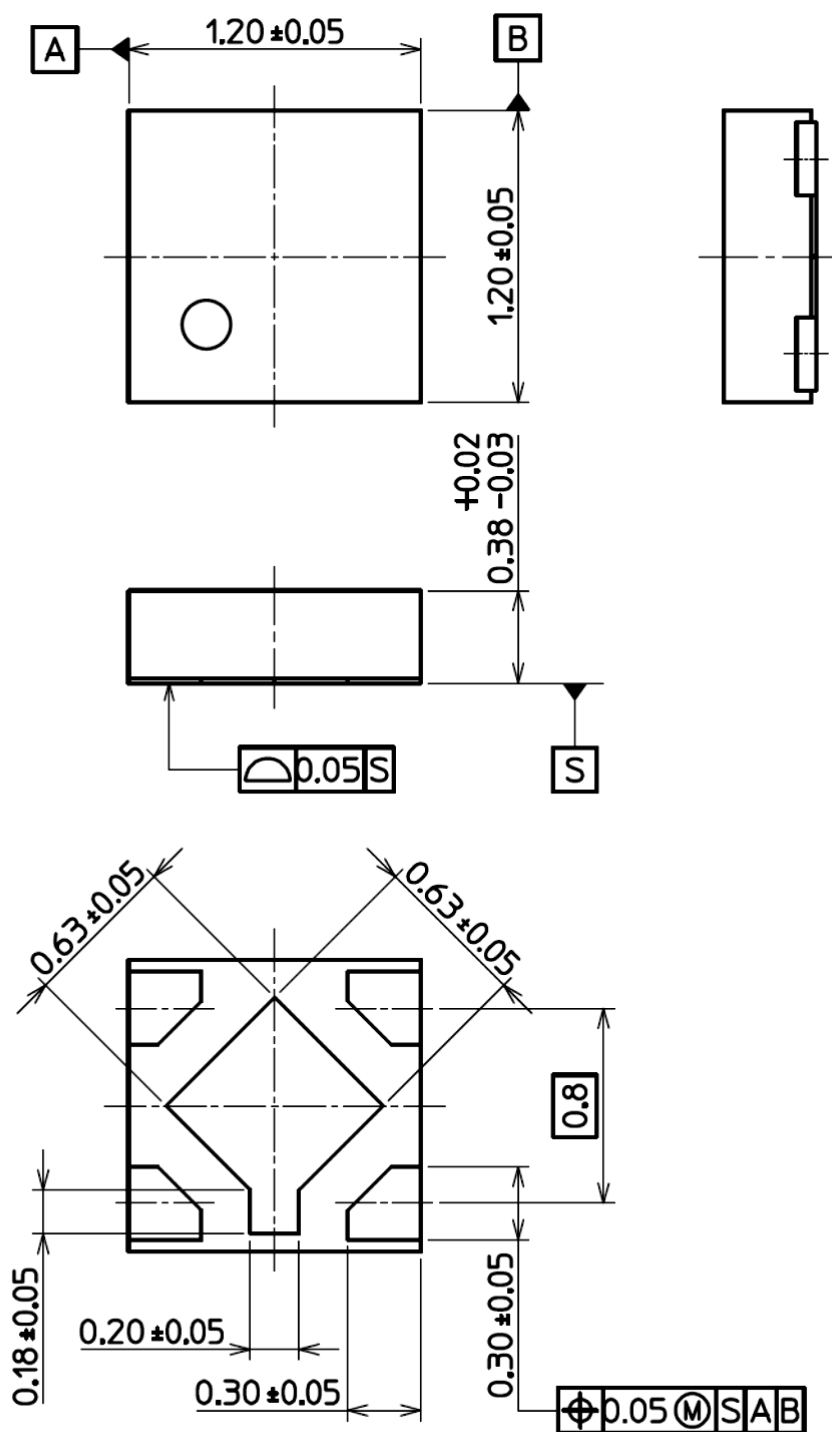
BOTTOM VIEW
