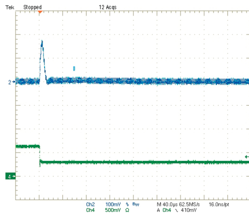
Step Load Transient Response (Vin=5V, Vout=3.3V, Cload=0, Iout=3A to 1.5A) Trace 2=Vout, 100 mV/div. Trace 4=Iout, 2.5A/div.
