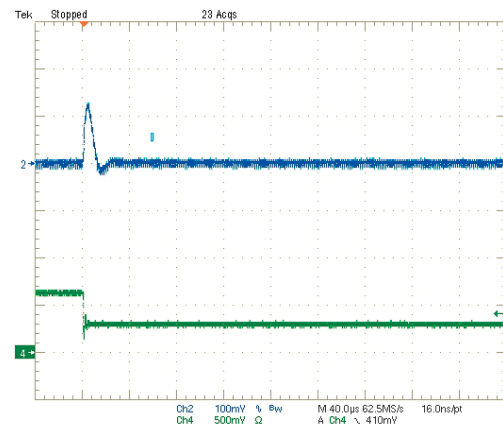
Step Load Transient Response (Vin=5V, Vout=1.0V, Clod=0, Iout=3A to 1.5A) Trace 2=Vout, 100 mV/div. Trace 4=Iout, 2.5A/div.
