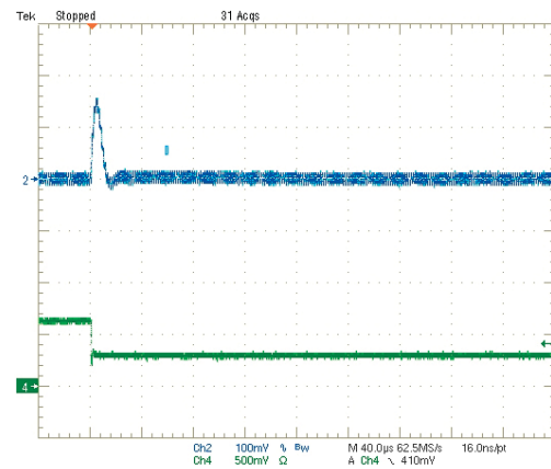
Step Load Transient Response (Vin=5V, Vout=2.5V, Clod=0, Iout=3A to 1.5A) Trace 2=Vout, 100 mV/div. Trace 4=Iout, 2.5A/div.
