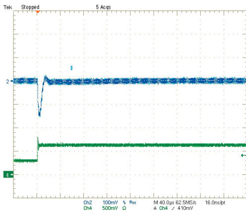
Step Load Transient Response (Vin=5V, Vout=2.5V, Clod=0, Iout=1.5A to 3A) Trace 2=Vout, 100 mV/div. Trace 4=Iout, 2.5A/div.
