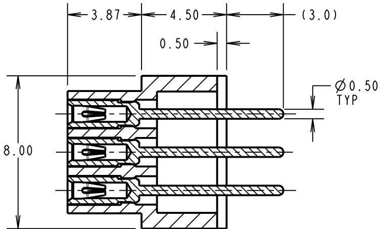
SECTION Y-Y
