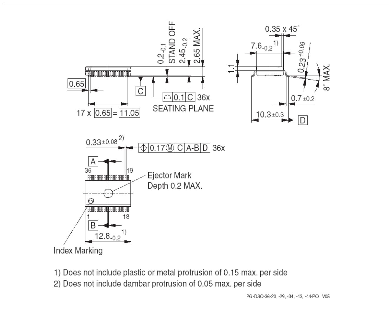
Figure 6-1 Package Dimensions
