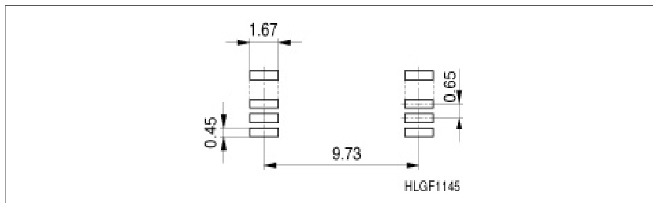
Figure 6-2 Recommended Footprint
