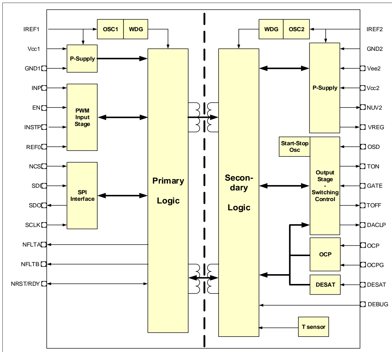
Figure 2-2 Block Diagram
