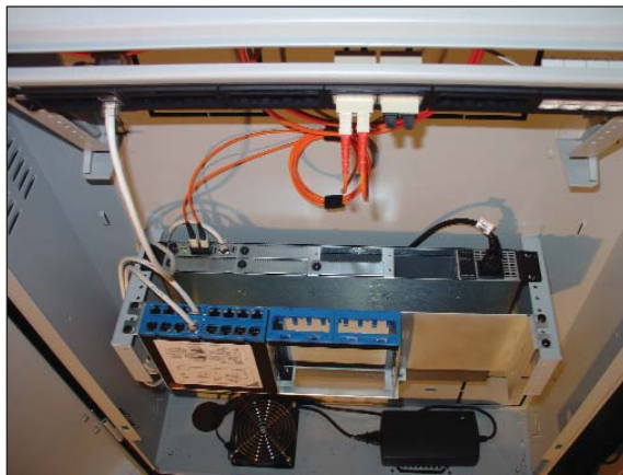
Figure 3. Top view and front view of chassis-based media converter and PoE midspan connected inside active wall mount zone enclosure
