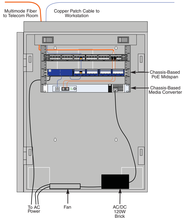
Figure 3. Top view and front view of chassis-based media converter and PoE midspan connected inside active wall mount zone enclosure
