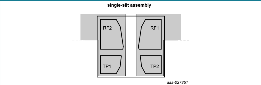
Figure 10. Single-slit assembly
