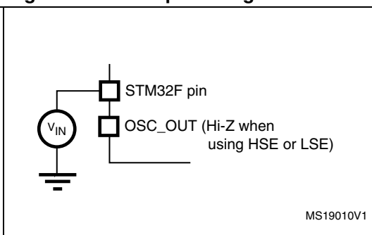
Figure 18. Pin input voltage
