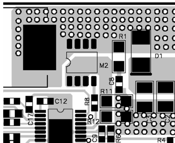
Figure 6—Layout Consideration
