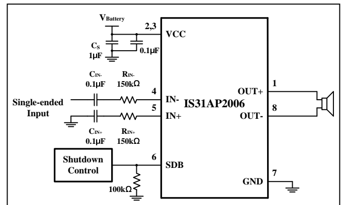
Figure 13 Typical Application Circuit with Single-Ended Input
