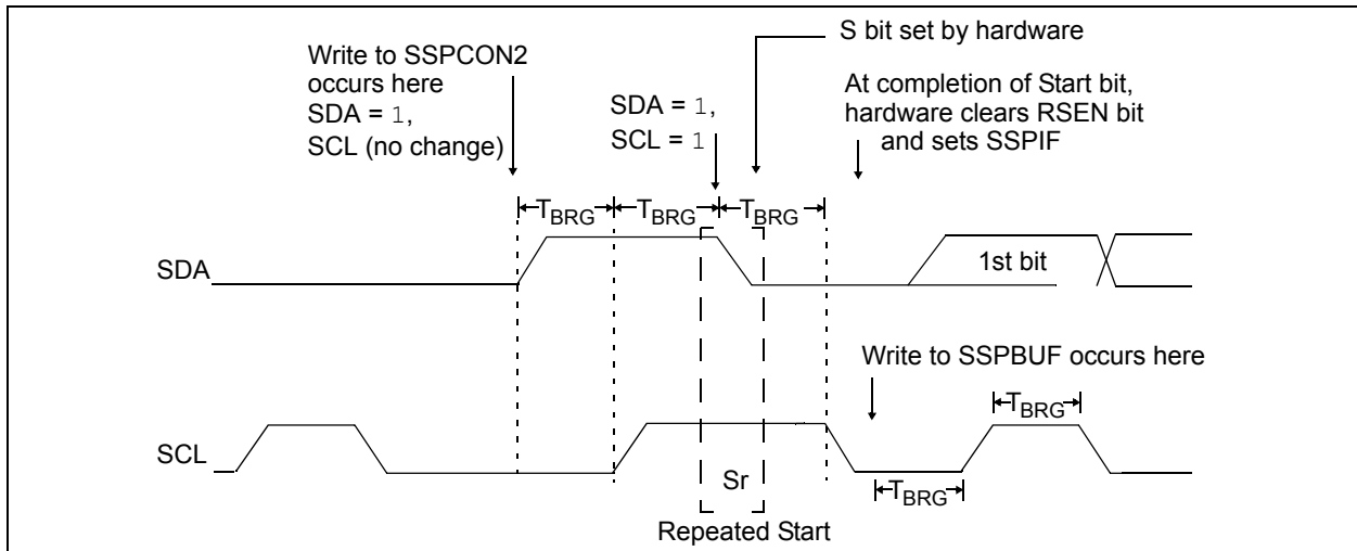
FIGURE 27-19: REPEAT START CONDITION WAVEFORM
