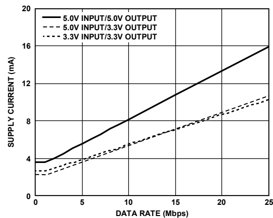
Figure 23. Typical I_{CHN} Supply Current per Forward Data Channel (15 pF Output Load)
