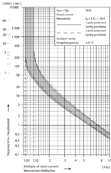
Tripping Characteristics I_n \ge 3 \dots < 18 A
