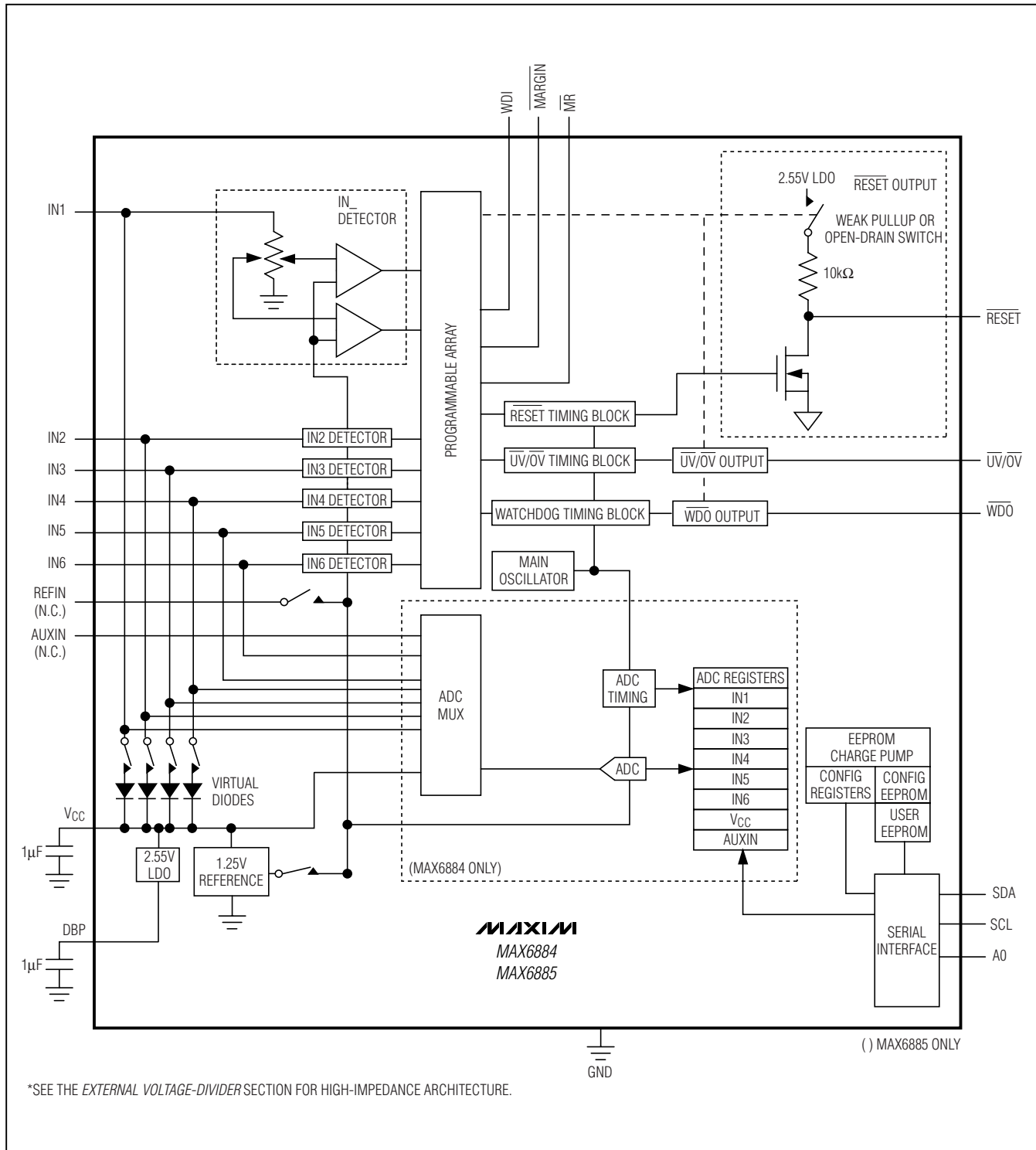
Functional Diagram
