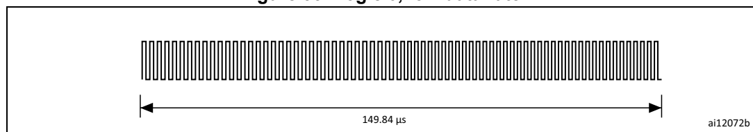
Figure 33. Logic 0, low data rate
