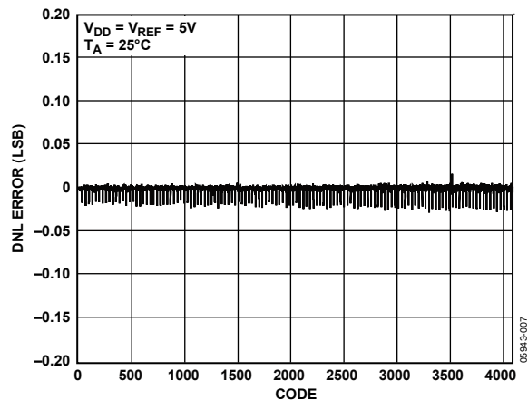
Figure 7. DNL AD5624
