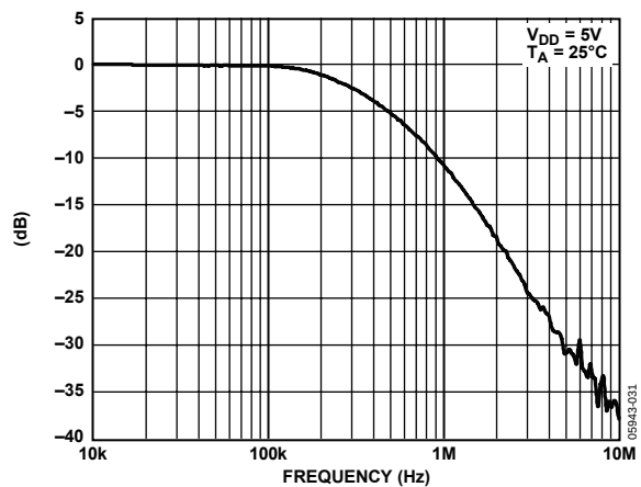
Figure 28. Multiplying Bandwidth
