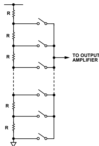
Figure 30. Resistor String
