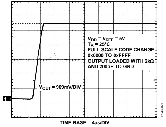
Figure 19. Full-Scale Settling Time, 5 V
