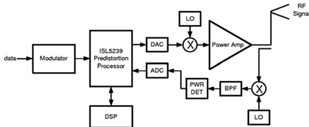
FIGURE 1. SYSTEM OVERVIEW
