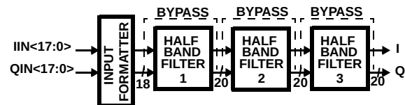
FIGURE 2. INPUT FORMATTER AND INTERPOLATOR BLOCK DIAGRAM
