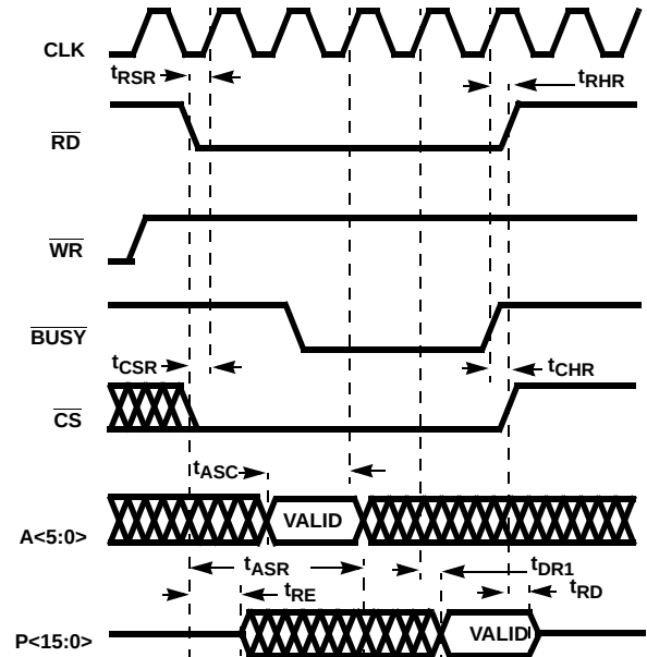
FIGURE 22. MICROPROCESSOR READ TIMING
