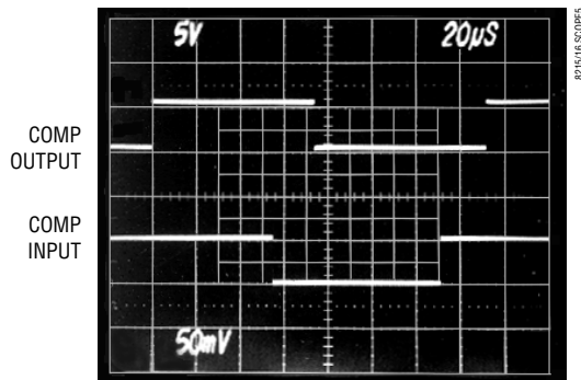
DIN COMPARATOR RESPONSE WITH 50mV OVERDRIVE
