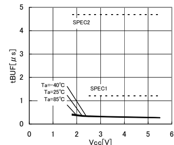
Fig.27 Bus release time before transfer start t_{BUF}
