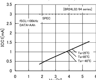
Fig.13 Current consumption at WRITE action ICC1 (fSCL=100kHz)
