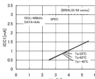
Fig.10 Current consumption at WRITE action ICC1 (fSCL=400kHz)
