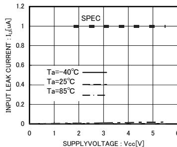
Fig.7 Input leak current I_{II} (A0,A1,A2,SCL,WP)
