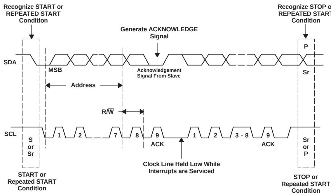
Figure 44. Bus Protocol
