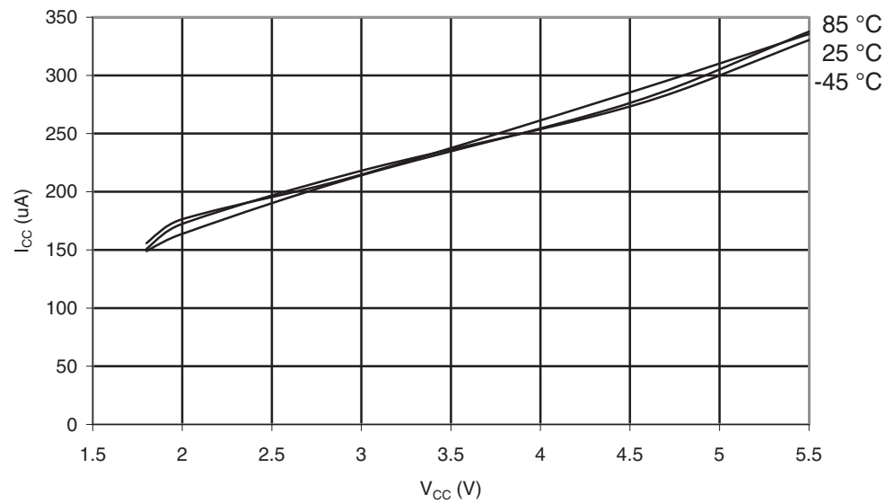
Figure 29-106. ATmega3290P: Active Supply Current with ADC at 1MHz vs. V_{CC}
