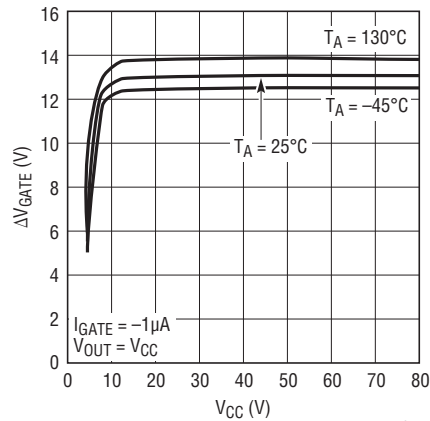
\Delta V_{GATE} vs V_{CC}
