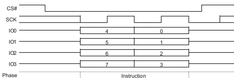
Figure 116. Software Reset Command Sequence QPI Mode
