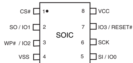
Figure 37. 8-Pin Plastic Small Outline Package (SOIC8)
