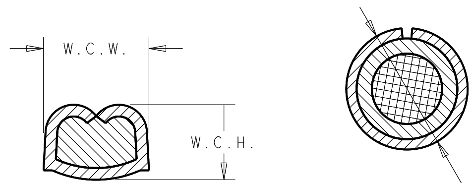
WIRE CRIMP DIMENSIONS INSULATION CRIMP DIMENSIONS
