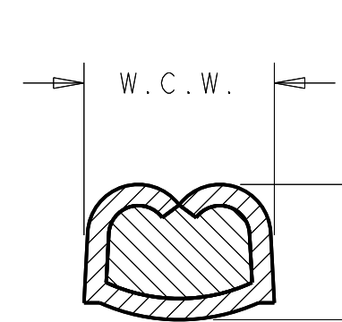
WIRE CRIMP DIMENSIONS INSULATION CRIMP DIMENSIONS
