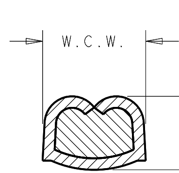
WIRE CRIMP DIMENSIONS
