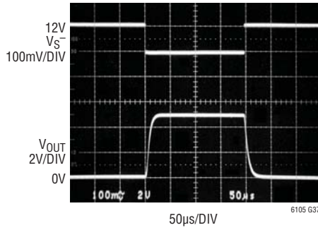
Step Response V_{SENSE} = 0V \text{ to } 100mV, C_L = 1000pF, V_S^+ = 12V
