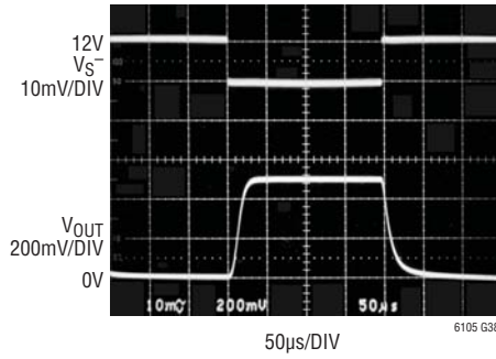
Step Response V_{SENSE} = 0V \text{ to } 10mV, C_L = 1000pF, V_S^+ = 12V
