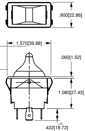
WITH .250 TAB TERMINALS AND FN BRACKET
