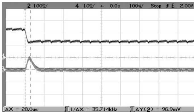
Step Load Transient Response (Vin=12V, Vout=3.3V, Cload=0, Iout=1A to 0.5A, Ta=+25°C.) Trace 2=Vout, 100 mV/div. Trace 4=Iout, 0.5A/div.
