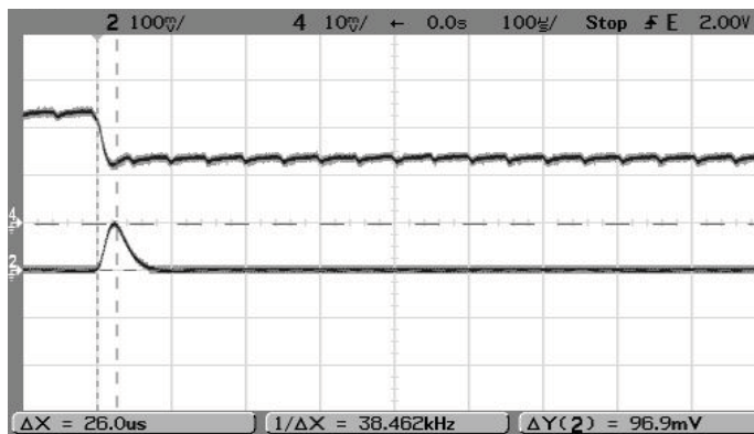
Step Load Transient Response (Vin=4.5V, Vout=3.3V, Cload=0, Iout=1A to 0.5A, Ta=+25°C.) Trace 2=Vout, 100 mV/div. Trace 4=Iout, 0.5A/div.
