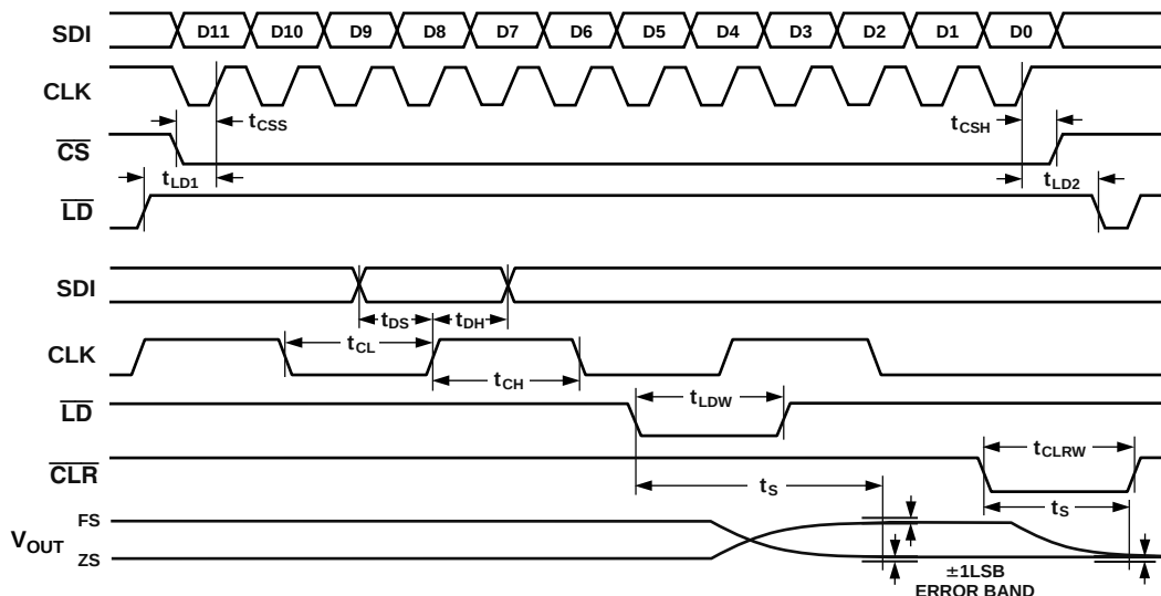
Figure 3. Timing Diagram
