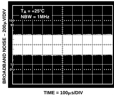
Figure 7. Broadband Noise
