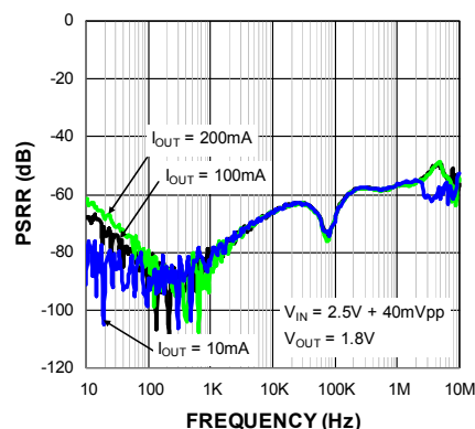
PSRR C_{OUT} = 1\mu\text{F}
