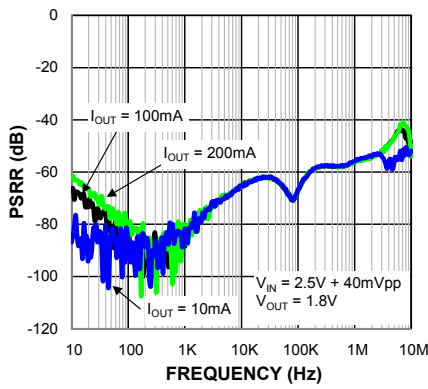
PSRR C_{OUT} = 0.47\mu F
