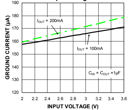
Ground Current vs. Input Voltage
