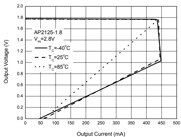
Figure 12. Current Limit
