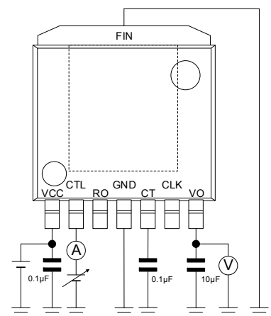
Measurement setup for Figure 11,12,13.
