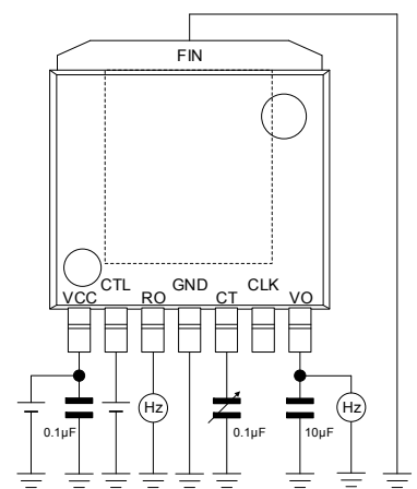
Measurement setup for Figure 19,20,21,22.
