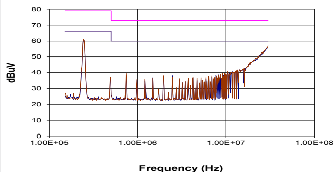
MTC1S2403SC
