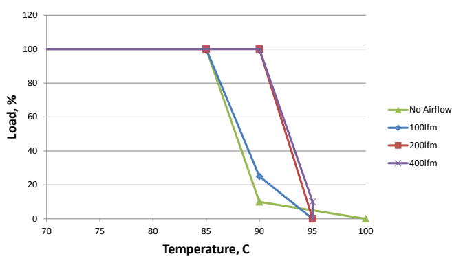
MTC1S2403SC - 36Vin
