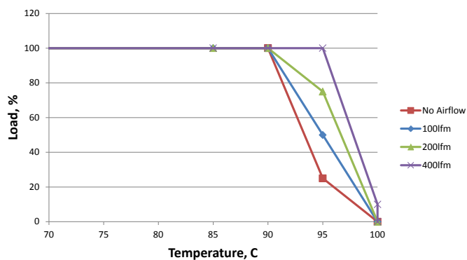
MTC1S1205SC - 12Vin
