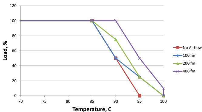
MTC1S1212SC - 12Vin
