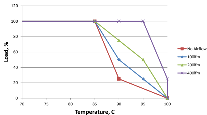
MTC1S1203SC - 12Vin
