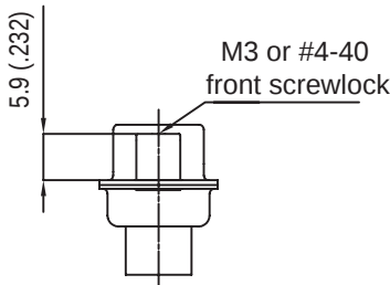
Fixed front female screwlock VF / VFM
