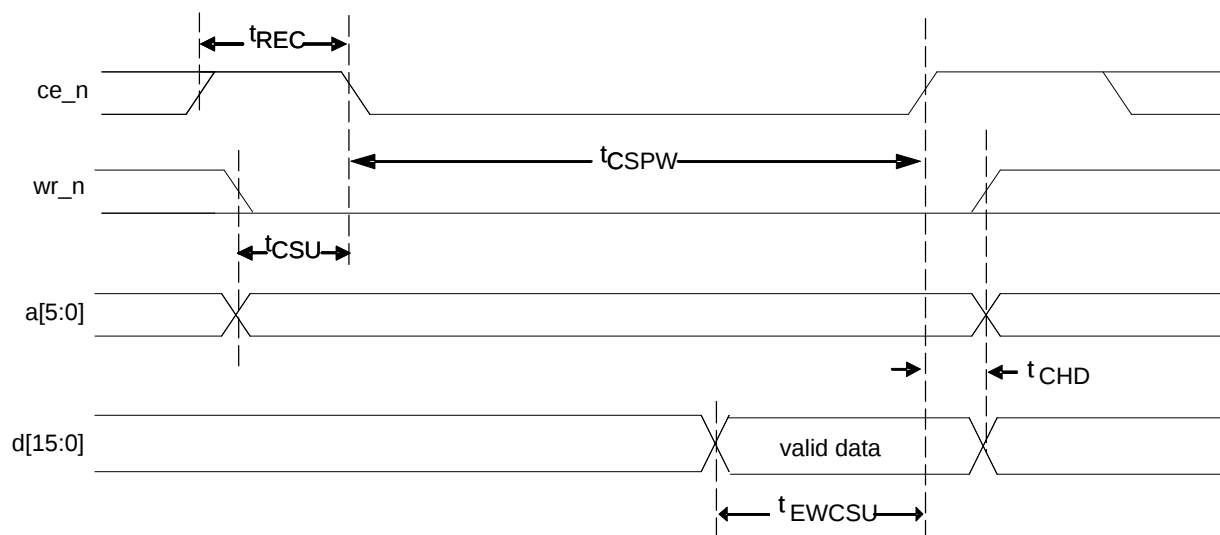
Figure 4-4. Write Operation – 2 pin control mode (rd_n tied low)
