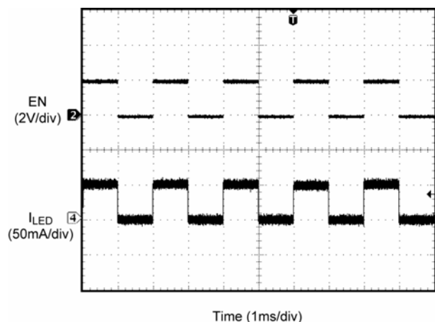
Figure 8. PWM Signal at 50% Duty Cycle ( I_{avg} = 25mA )
