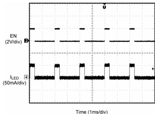
Figure 7. PWM Signal at 20% Duty Cycle ( I_{avg} = 10mA )
