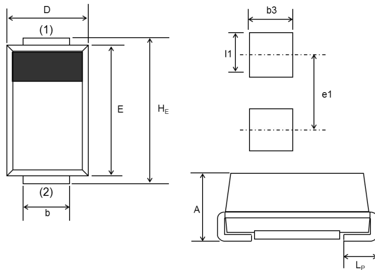
DO-214AC(SMA), (PMDS)
