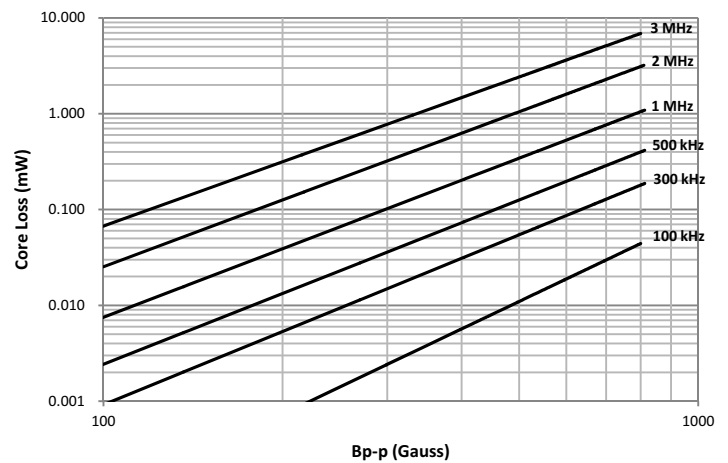
MPI2512V2-2R2-R
