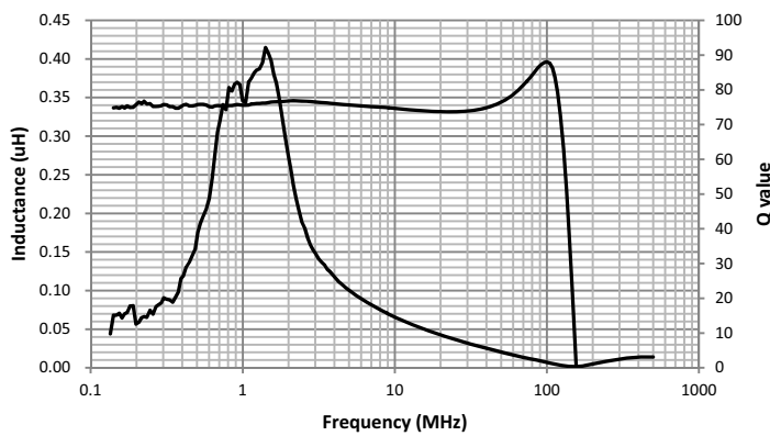
MPI2512V2-R33-R
