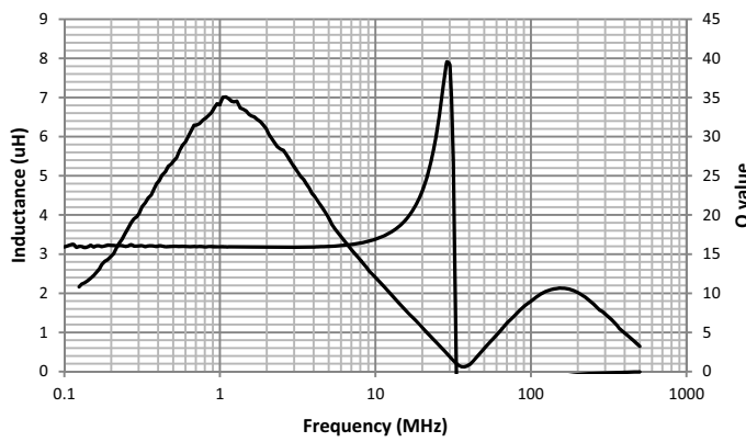
MPI2510V2-3R3-R
