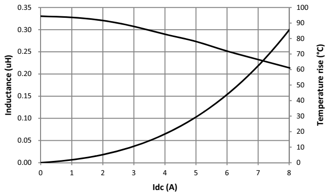
MPI2512V2-R33-R
