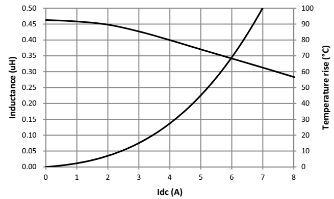
MPI2512V2-R47-R
