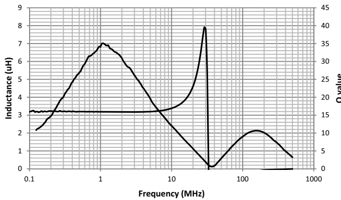
MPI2510V2-3R3-R
