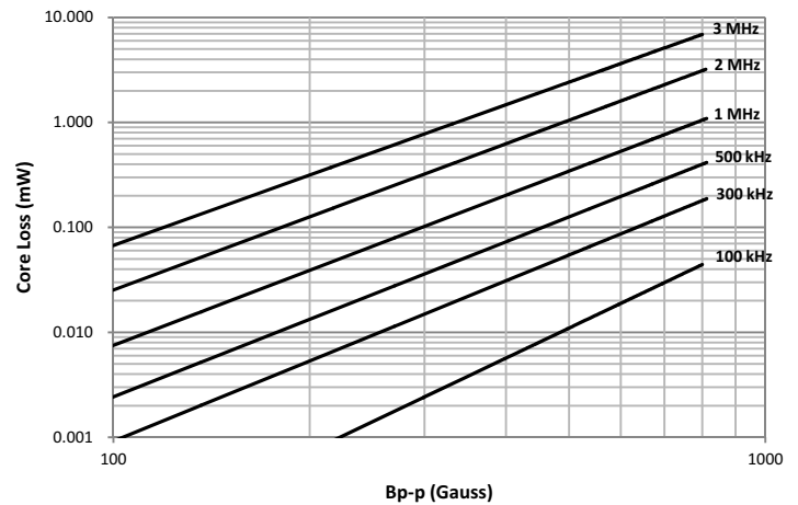
MPI2512V2-2R2-R
