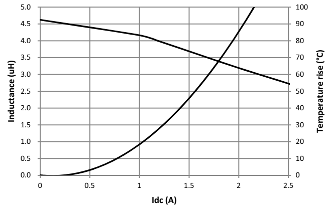
MPI2510V2-4R7-R
