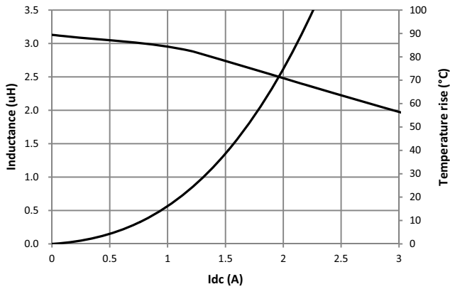
MPI2510V2-3R3-R
